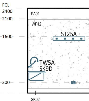
9 ELEVATION DETAIL 1 : 50
