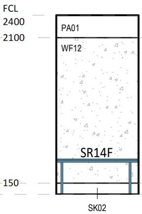
2 ELEVATION DETAIL 1 : 50
