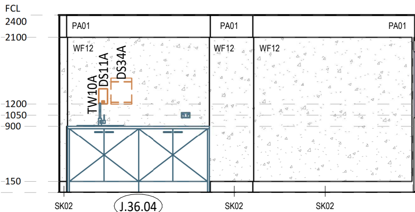
4 ELEVATION DETAIL 1 : 50
