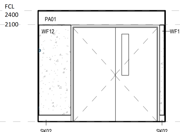
6 ELEVATION DETAIL 1 : 50
