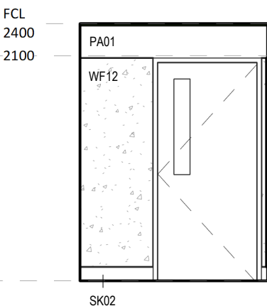
7 ELEVATION DETAIL 1 : 50
