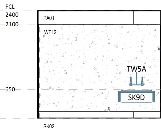
8 ELEVATION DETAIL 1 : 50
