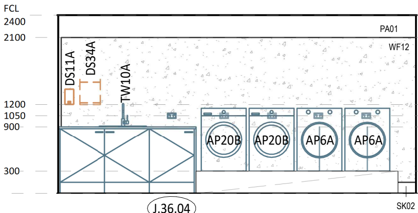
3 ELEVATION DETAIL 1 : 50
